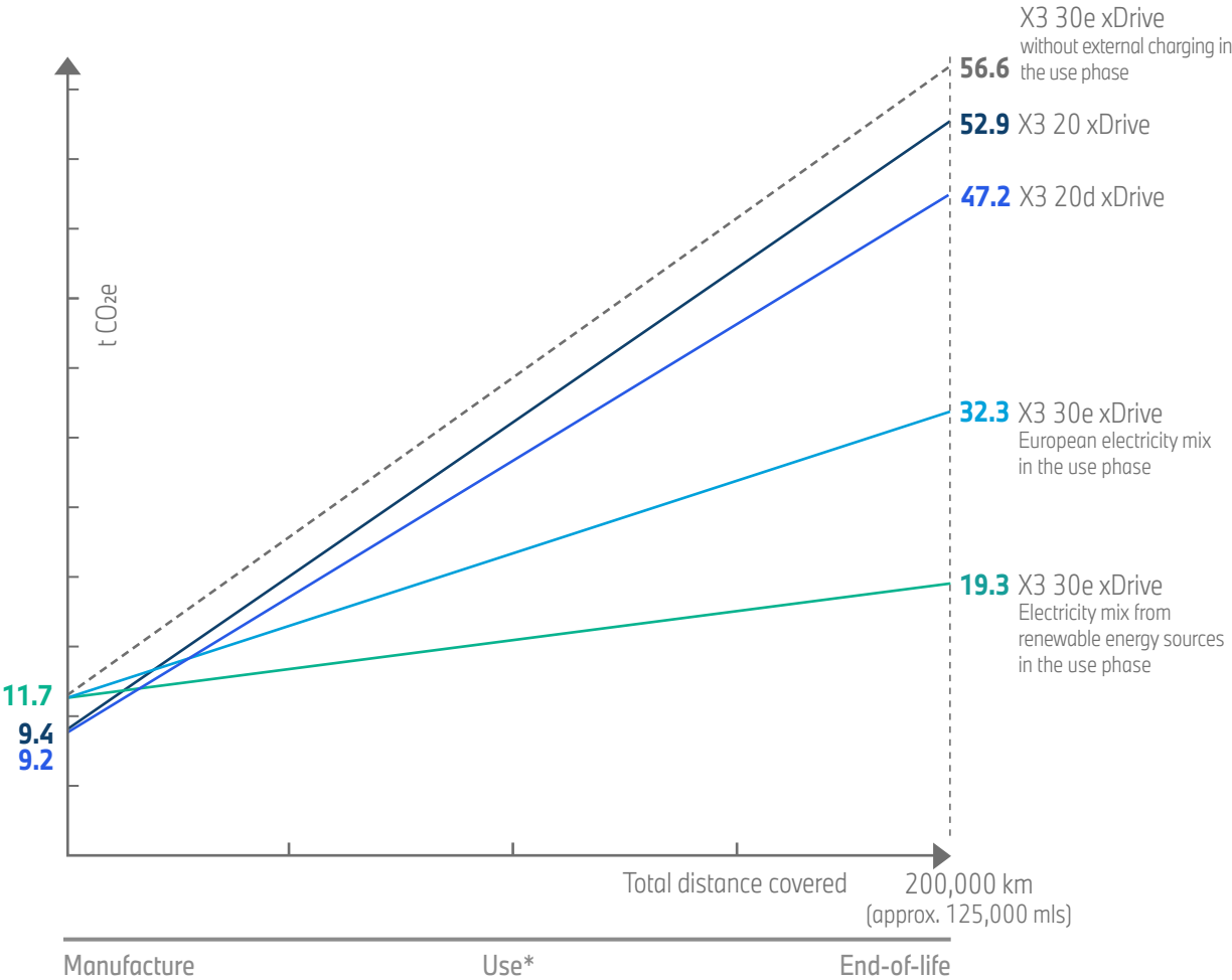
Fig. 4: Comparison of the CO 2 equivalents of the BMW X3 30e xDrive in relation to diesel and petrol models
