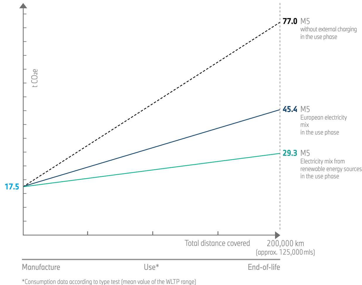
Fig. 4: Comparison of the CO 2 equivalents of the BMW M5 depending on charging behavior and energy mix.
